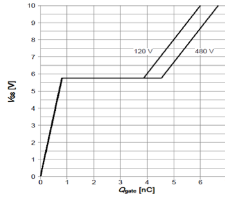
Figure 8: Gate-Charge Characteristics
