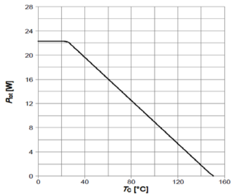
Figure 3: Power Dissipation
