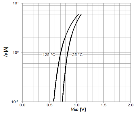
Figure 7: Body-Diode Characteristics
