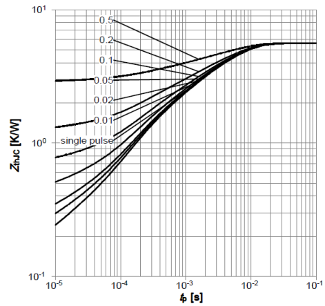
Figure 12: Sing Pulse Power Rating Junction to Case
