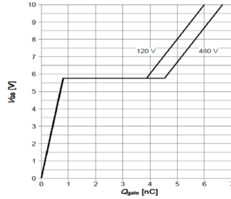
Figure 8: Gate-Charge Characteristics
