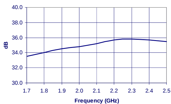
Output IP3
