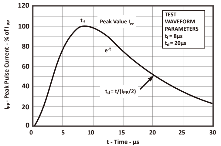
Pulse Waveform
