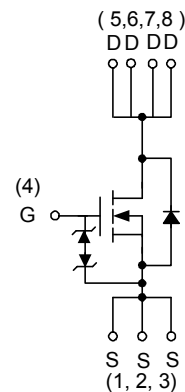
N-Channel MOSFET
