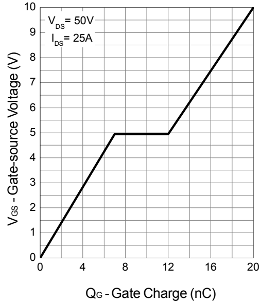
Gate Charge
