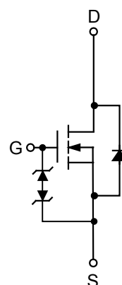
N-Channel MOSFET
