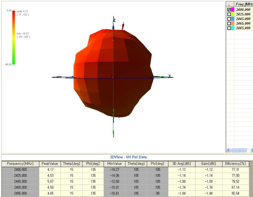
Figure 1.3: Partron SDBTPTR3015 Antenna Gain Performance
