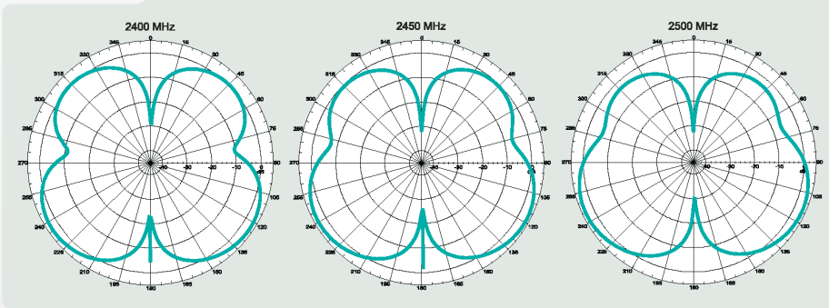
Figure 1.4: Pulse W1027 Antenna Gain Performance
