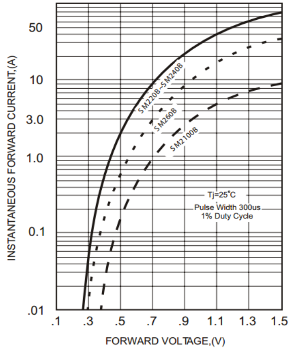
FIG.2-TYPICAL FORWARD CHARACTERISTICS
