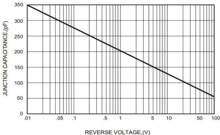
FIG.4-TYPICAL JUNCTION CAPACITANCE
