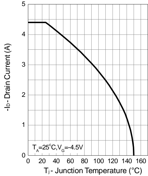
Drain Current
