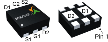
DFN2x2-6
