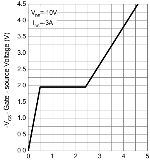
Gate Charge
