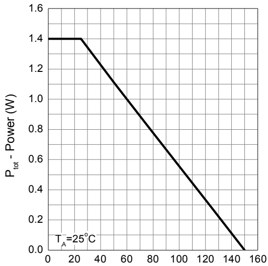
Power Dissipation
