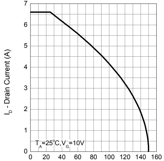
Drain Current
