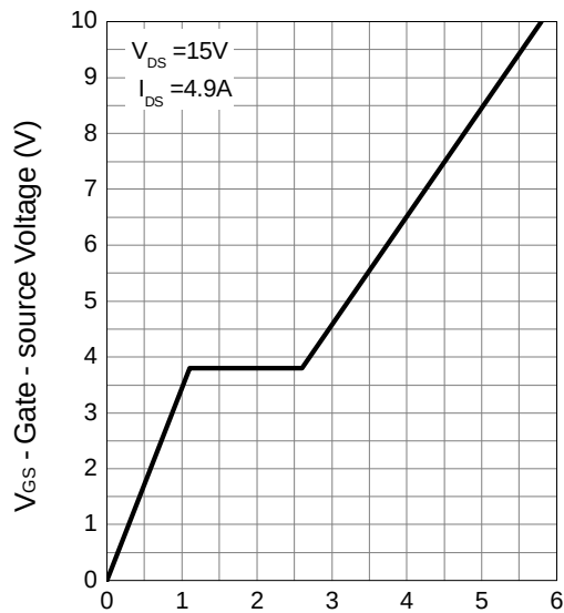
Gate Charge
