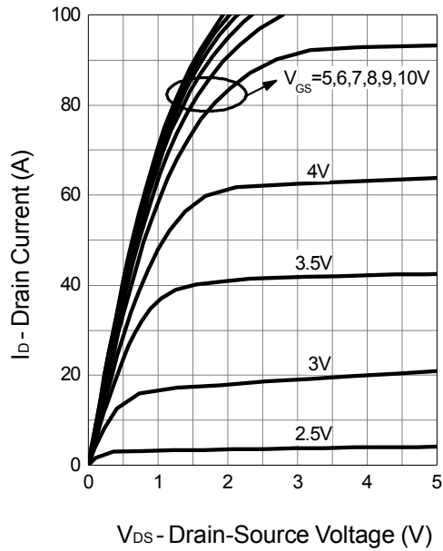
Output Characteristics
