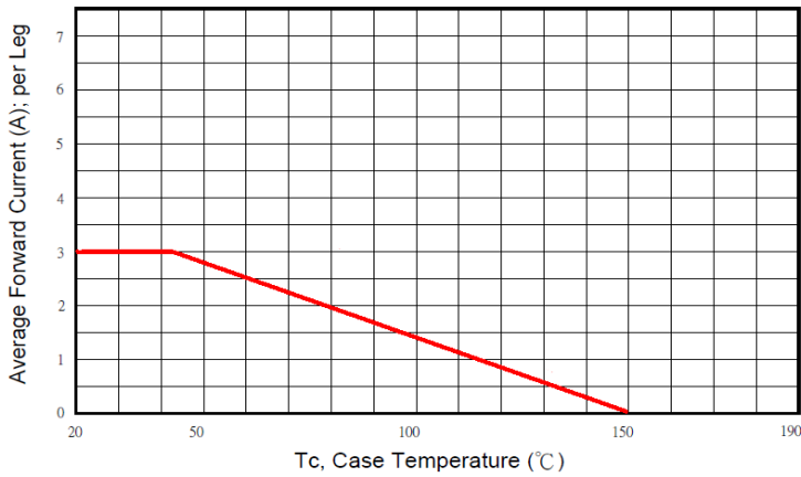
Typical Forward Current Derating Curve
