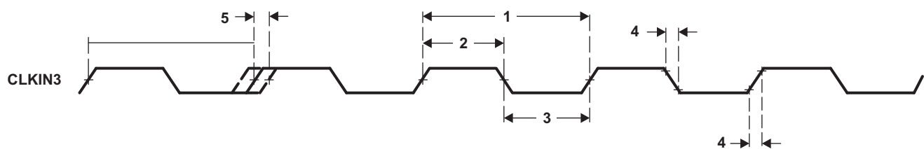
Figure 7-37. CLKIN3 Timing
