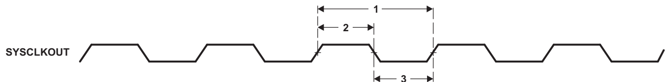
Figure 7-24. SYSCLKOUT Timing
