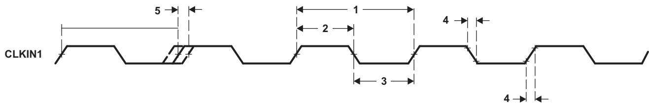
Figure 7-23. CLKIN1 Timing
