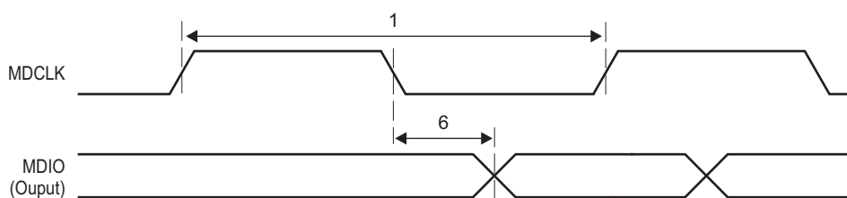
Figure 7-61 MDIO Output Timing
