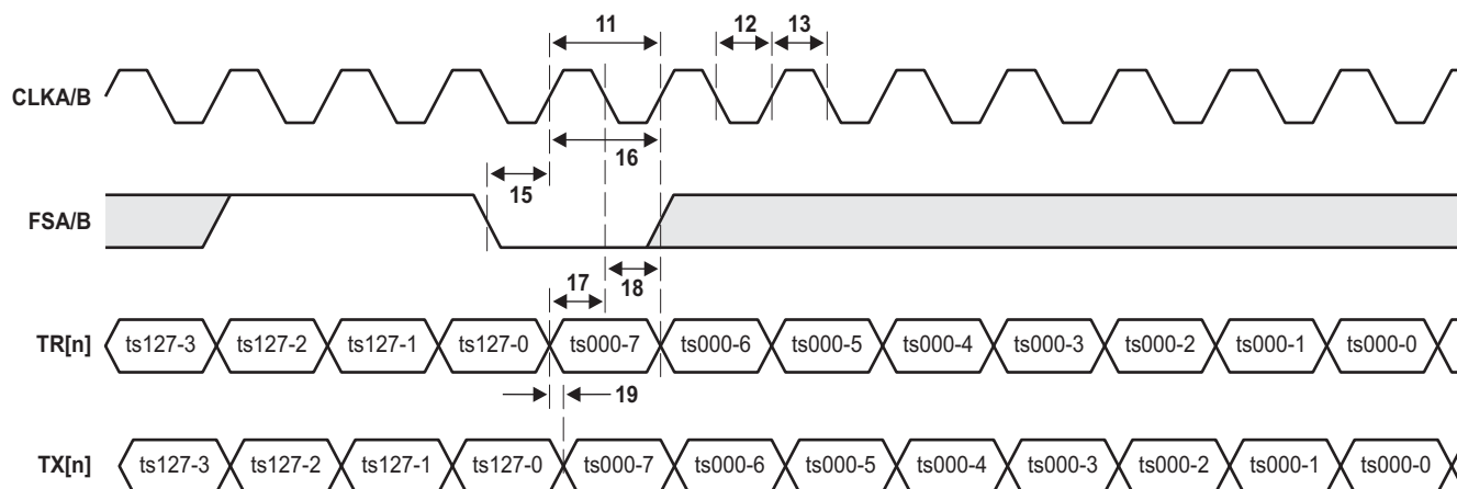
Figure 7-52 TSIP 1x Timing Diagram (1)
