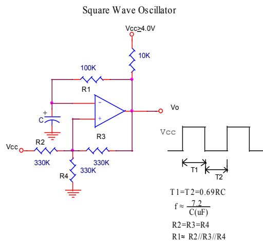
Fig 6.Square wave oscillator
