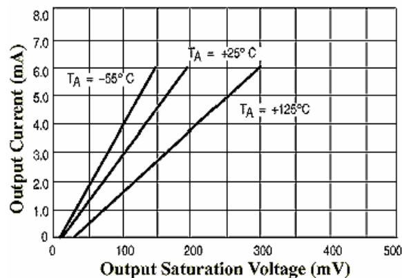
Fig 3. Output sink current versus output saturation voltage
