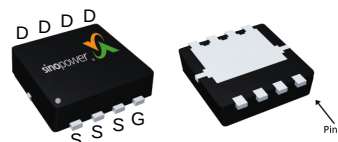
DFN3.3x3.3-8
