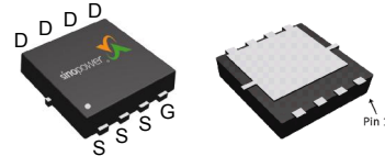
DFN3.3x3.3D-8_EP
