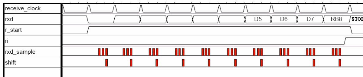
Fig. 8-6: Receive modes 2 and 3
