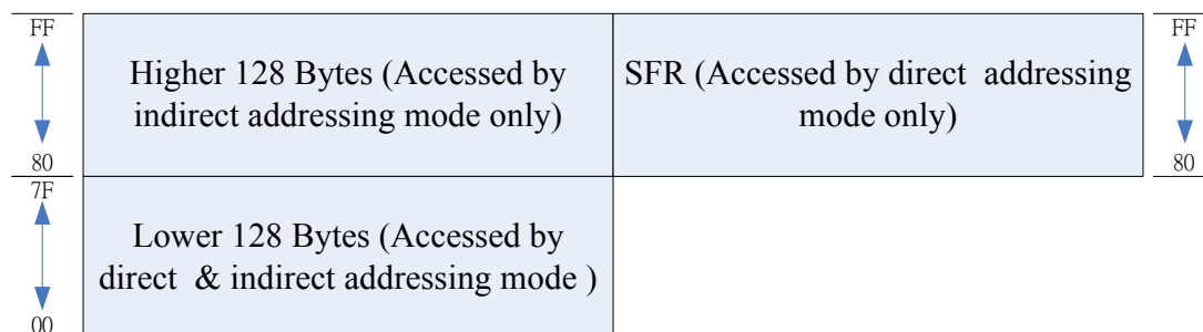
Fig. 3-4: RAM architecture
