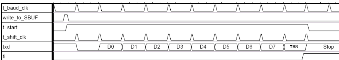
Fig. 8-5: Transmit modes 2 and 3
