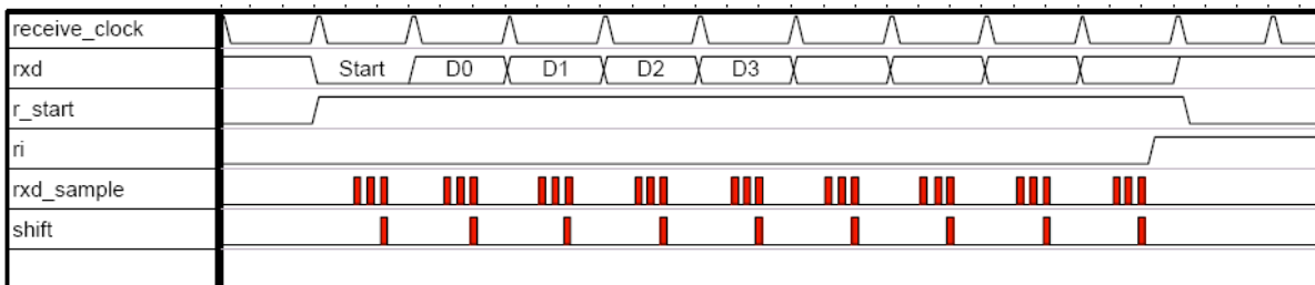
Fig. 8-4: Receive mode 1
