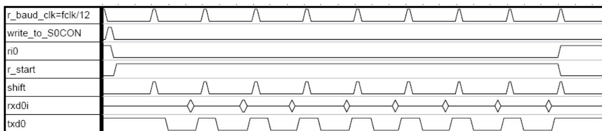
Fig. 8-2: Receive mode 0
