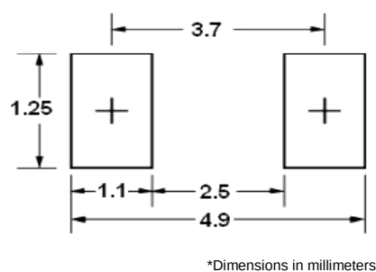
FIG. 6-MOUNTING PAD LAYOUT
