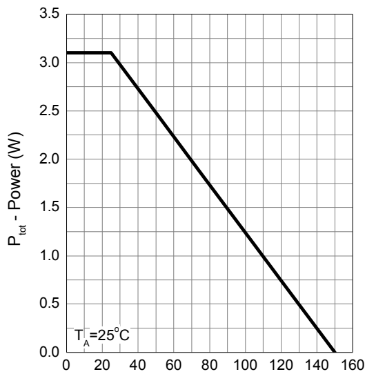
Power Dissipation
