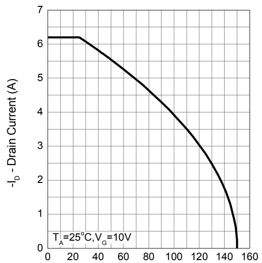
Drain Current
