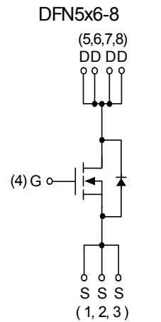
N-Channel MOSFET
