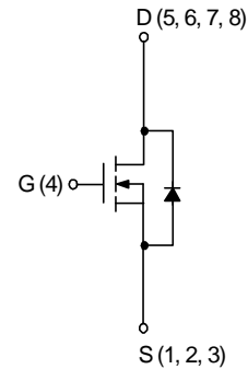
N-Channel MOSFET
