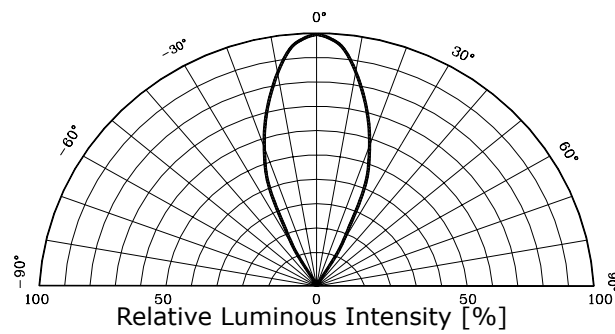
Fig. 5 Radiation Diagram
