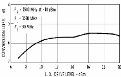
Conversion Loss
