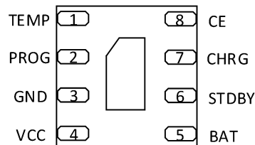
DFN2X2-8L
