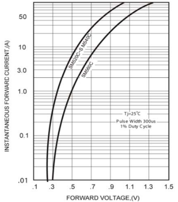
FIG.2-TYPICAL FORWARD CHARACTERISTICS
