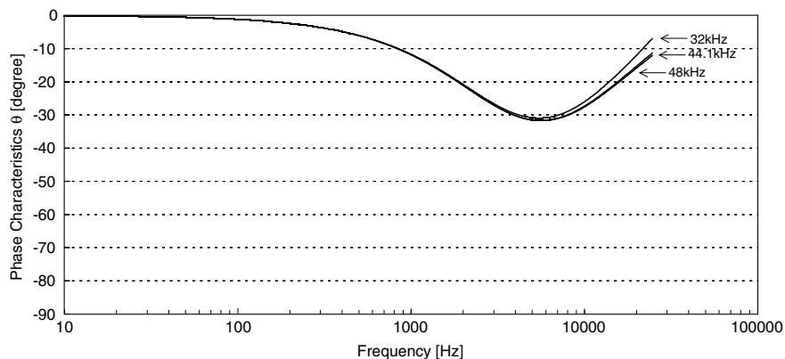
Figure 3. Deemphasis filter phase characteristics
