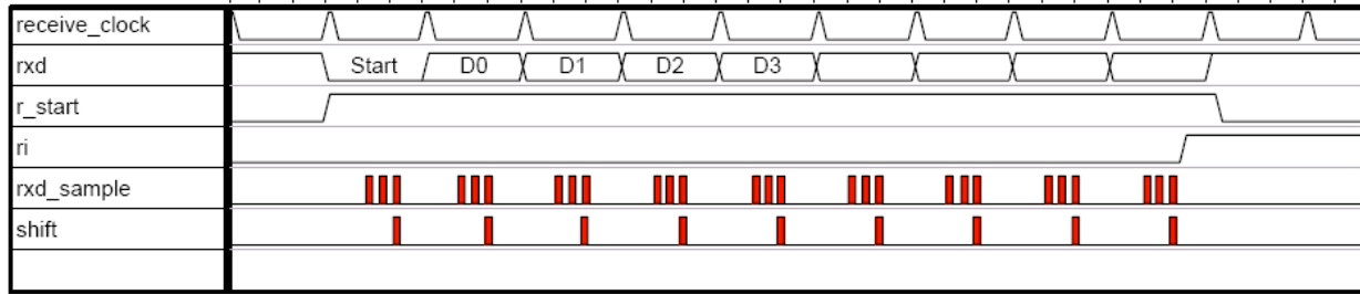
Fig. 8-4: Receive mode 1
