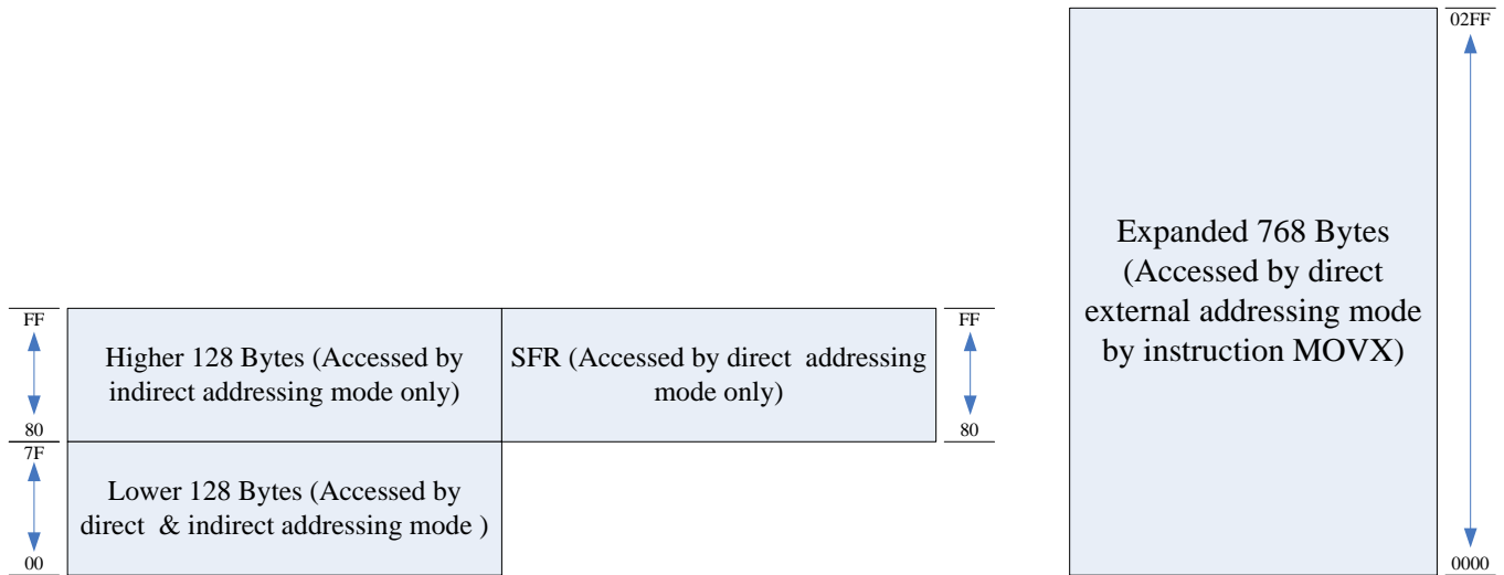
Fig. 3-2: RAM architecture
