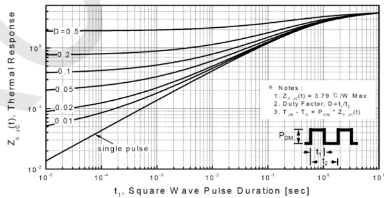
Figure 11. Transient Thermal Response Curve for WGF5N60
