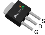
Top View of TO-251S
