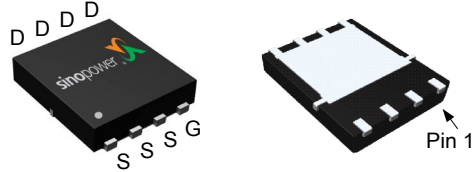
DFN5x6-8
