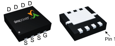
DFN3.3x3.3-8
