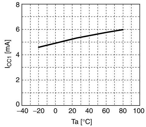
Figure 2. Current consumption 1 vs. Ambient temperature
