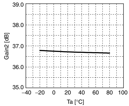
Figure 5. Output gain vs. Ambient temperature (at 10Hz input frequency)
