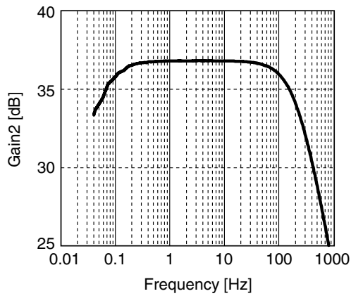
Figure 4. Output gain vs. Frequency
