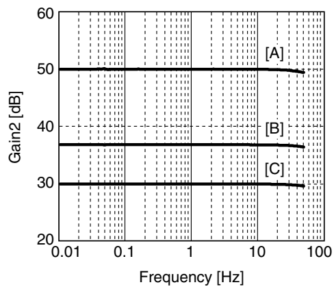
Figure 6. Output gain vs. Frequency (when changing output gain setting *1 )
