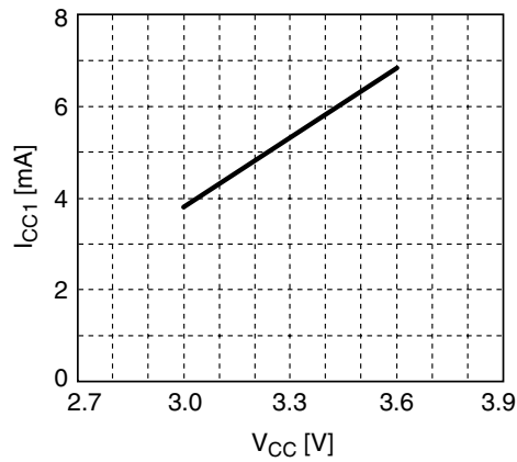
Figure 1. Current consumption 1 vs. Supply voltage
