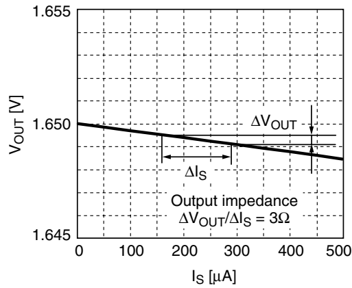
Figure 7. Output current vs. Output voltage *1 (VSIG_OUT1, VSIG_OUT2 pins)
