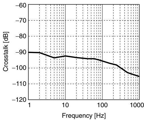
Figure 9. Crosstalk vs. Frequency *3
