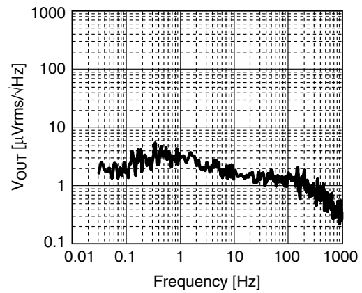
Figure 8. Output noise vs. Frequency *2
