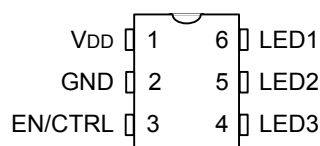
SM6803 SOT-26 / TSOP 6
