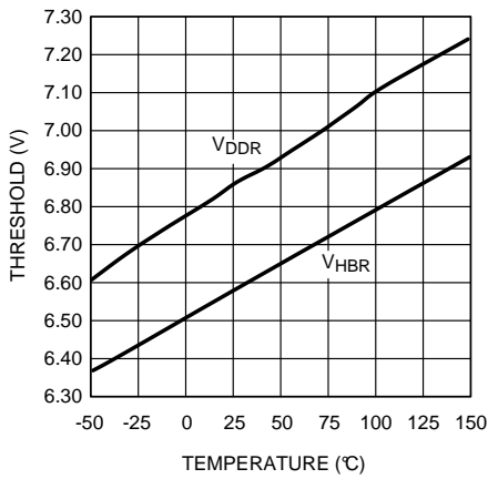
Figure 9. Undervoltage Rising Threshold vs Temperature
