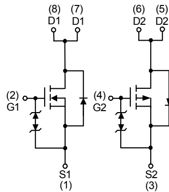
N-Channel MOSFET
