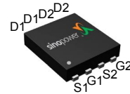
Top View of DFN3x3C-8
