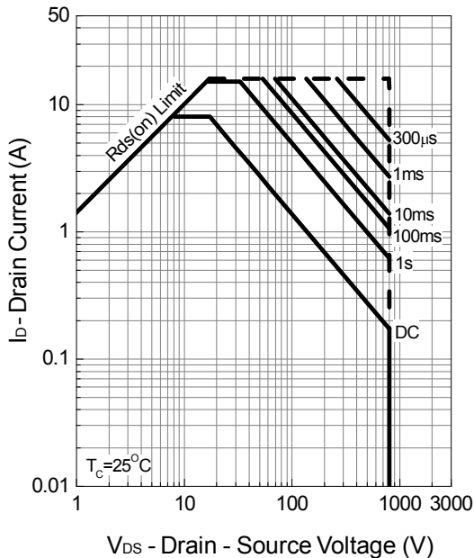
Safe Operation Area : TO-220/TO-247
