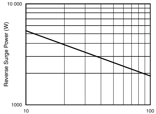
Figure 4. Reverse Power Capability
