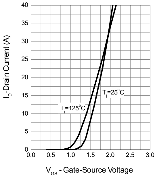
Transfer Characteristics
