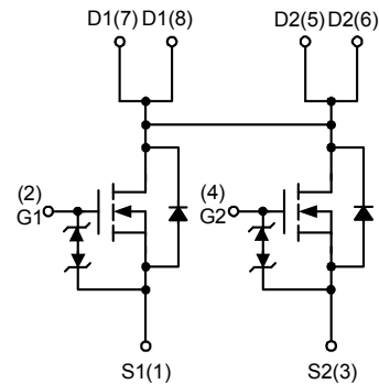
N-Channel MOSFET
