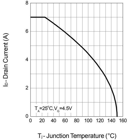
Drain Current
