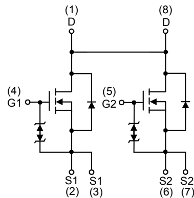
N-Channel MOSFET
