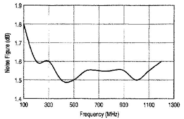
Noise Figure
