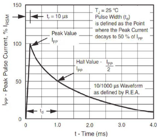
Figure 3. Pulse Waveform
