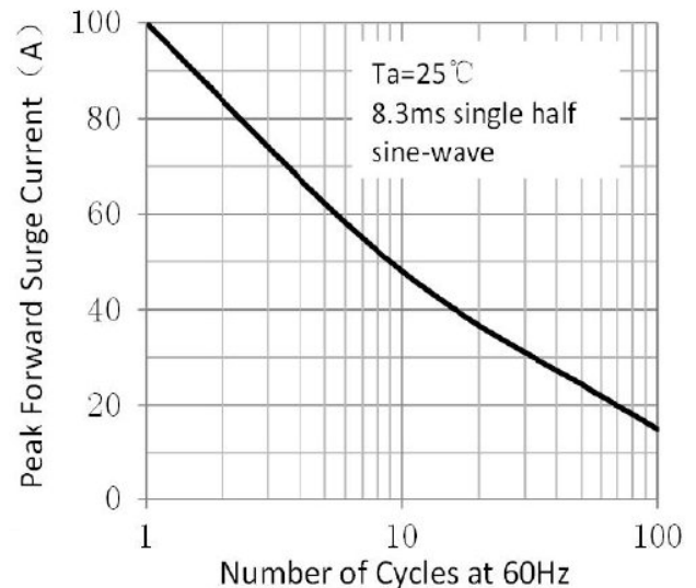
Figure 4. Maximum Non-Repetitive Peak Forward Surge Current
