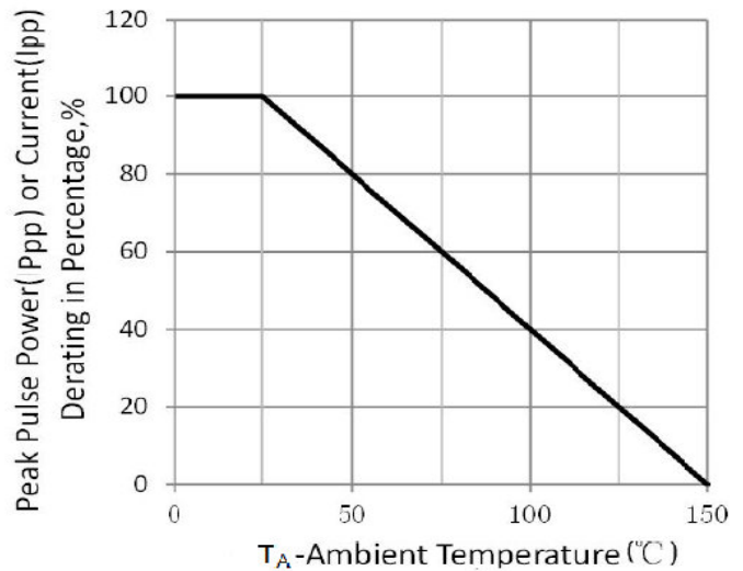
Figure 2. Pulse Power vs ambient temperature
