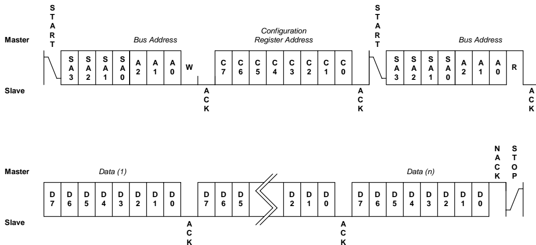
Figure 14 – Register Read
