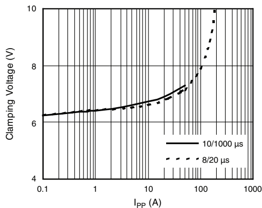
Fig. 4 - Clamping Voltage vs. Peak Pulse Current ( T_J initial = 25 ^\circ\text{C} )
