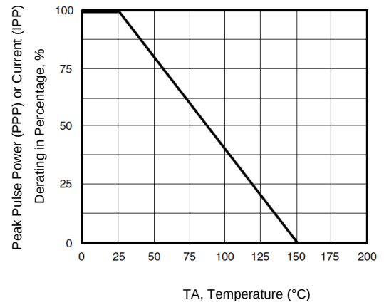
Fig.2 DERATING CURVE
