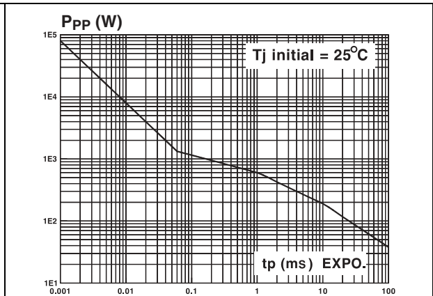
Figure 2. Peak pulse power versus exponential pulse duration.
