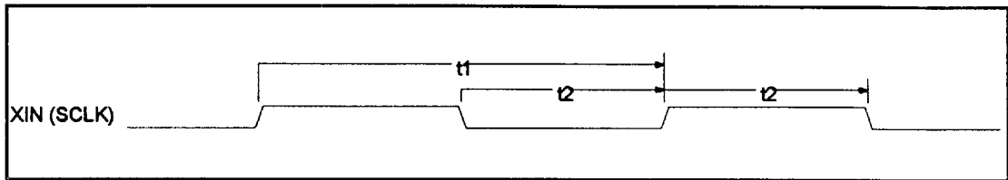
FIGURE 29 - CLOCK TIMING
