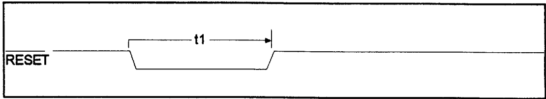
FIGURE 28 - RESET TIMING
